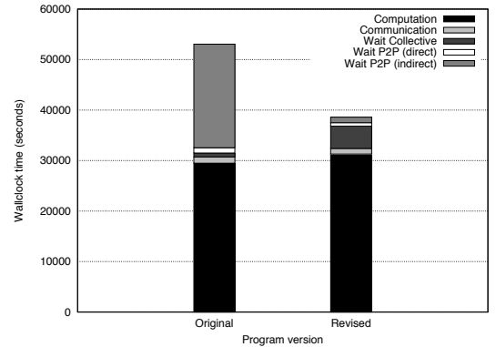
Fig. 11. Runtime composition and quantitative comparison of the original versus the revised version of Illumination . In the revised version, the indirect waiting time was significantly reduced and wait states were partially shifted from point-to-point to collective communication. A slight increase in computation time was caused by additional memory copies needed in context of the switch to non-blocking communication.
