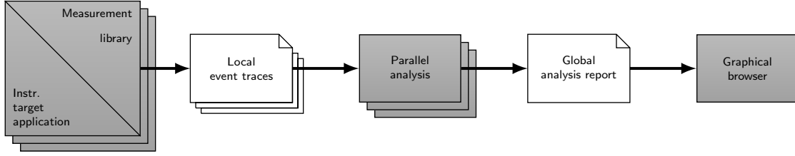
Fig. 1. Scalasca's parallel trace-analysis workflow. Gray rectangles denote programs and white rectangles with the upper right corner turned down denote files. Stacked symbols denote multiple instances of programs or files running or being processed in parallel.
