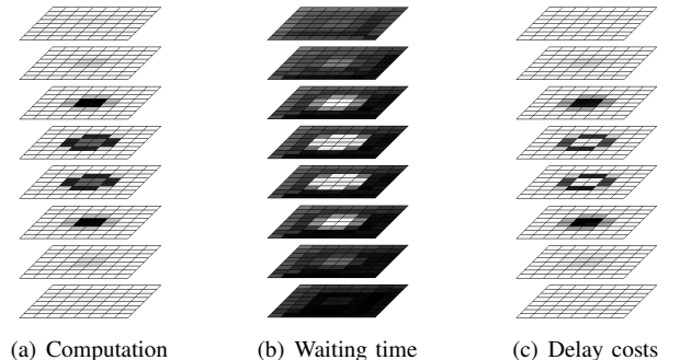
Fig. 9. Distribution of computation time, waiting time, and total delay costs in Zeus-MP/2 across the three-dimensional computational domain.
