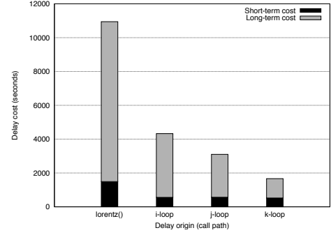
Fig. 8. Short- and long-term costs of delays in four critical call paths of Zeus-MP/2.
